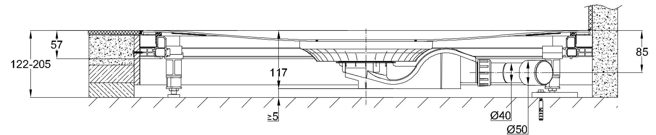
Representation Universal installation system with waste fitting BetteAir 50 – 0.6 l/s, with water drainage on the side, standard-compliant water seal depth 50 mm to EN 274
